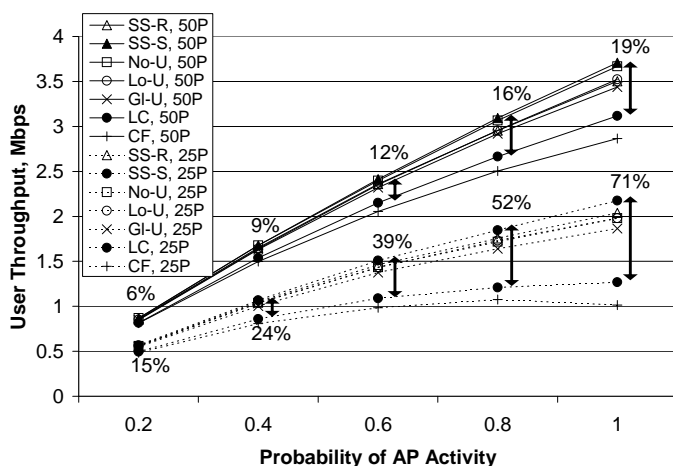
Fig. 5. 50 and 25 percentiles of users' throughputs (50P and 25P) respectively, including both downlink and uplink traffic, for 400 users on a 10-by-10 uniform AP layout with 10 rogues. Vertical arrows and numbers besides the arrows depict the gains of SS-S over LC in percents (some arrows are omitted when the associated gains are relatively small).
