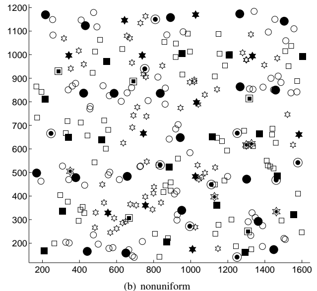
Fig. 6. Frequency allocation examples for 49 APs on a 7-by-7 nonuniform or uniform topology. Three kinds of objects (squares, stars, and circles) signify three orthogonal frequency channels. Filled back objects denote 49 APs; hollow objects denote 196 users; double-layered objects with inner part filled with black denote 20 rogues. The units of X and Y axes are meters.
