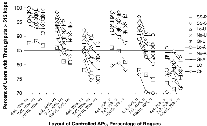
Fig. 4. Percent of users that have throughputs higher than 512 kbps. The x-axis represents the layout of controlled APs and the percentage of rogue APs compared to the controlled APs. Nonuniform and uniform AP layouts are denoted 'nu' and 'u', respectively.
